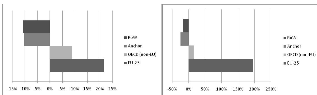
Figure 4: Net-trade flows as a percentage of domestic resource extraction (total, metal ores), in 2000
