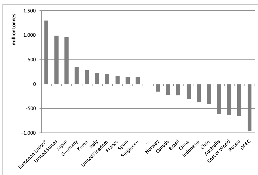
Figure 5: Physical trade balance (PTB) of different countries (total), in 2000
