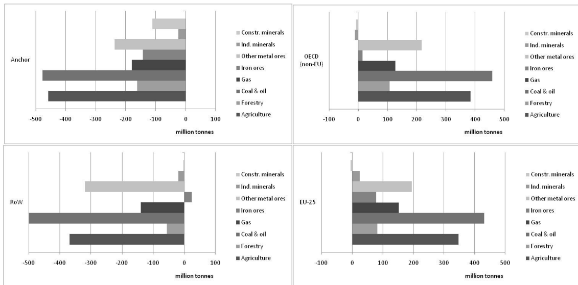
Figure 3: Physical trade balance (PTB) in four different world regions for eight material categories, in 2000
