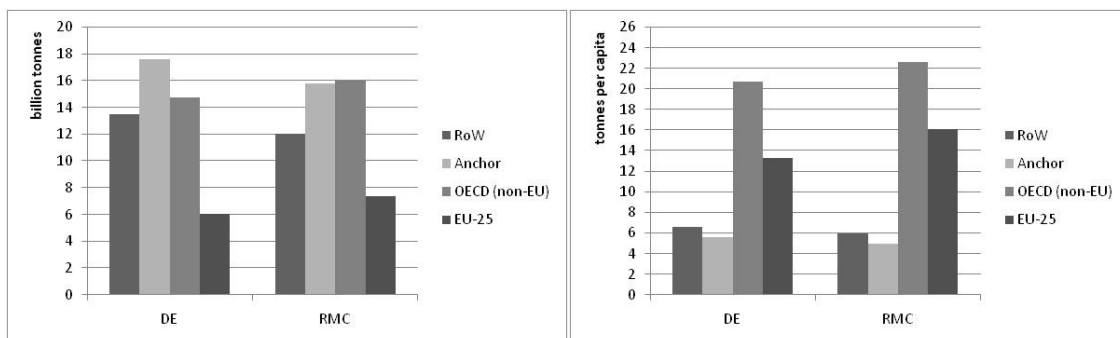
Figure 2: Domestic extraction (DE) and raw material consumption (RMC) in different world regions (total, per capita), in 2000
